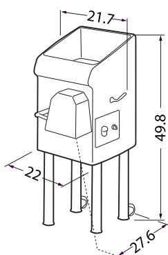
Dimensions TX98 on legs
