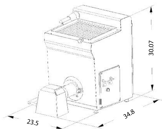
Dimensions TX98 Auto
