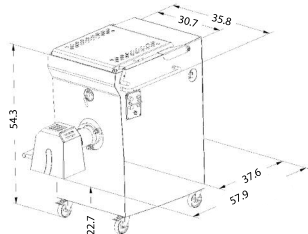
Dimensions TX52 ML
