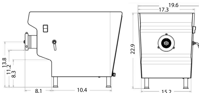
Dimensions TX22
