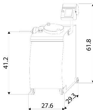
Dimensions TORSADO
