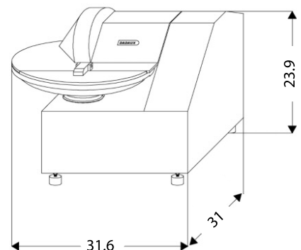
Dimensions TITANE 23
