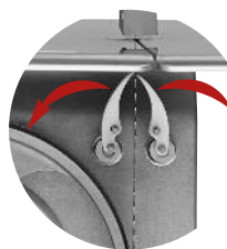
Spring-loaded scraper to ensure efficiency. It is retractable for easy blade placement and cleaning
