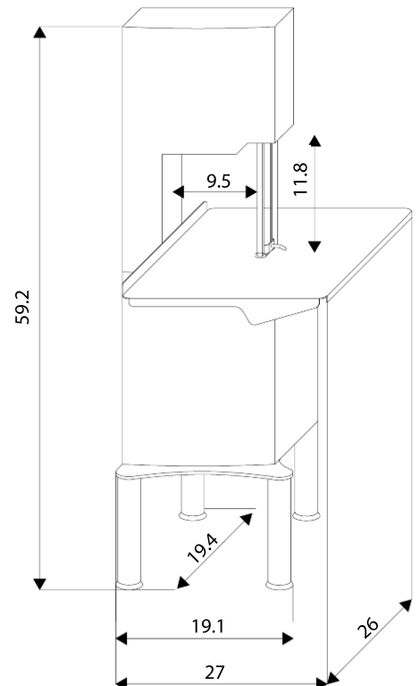
Dimensions SX300 & SX300-1P
