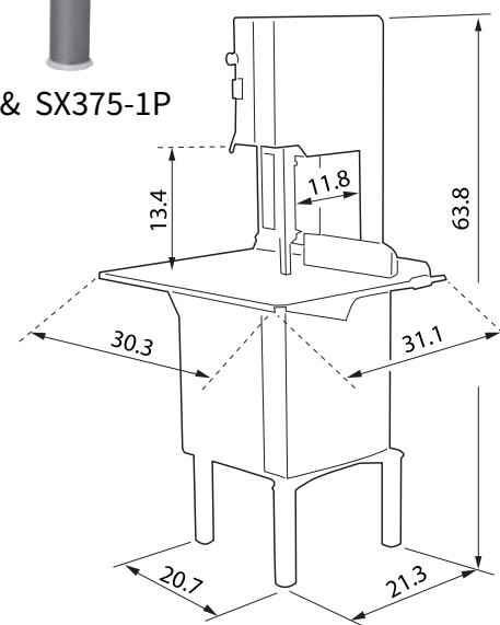
Dimensions SX375 & SX375-1P
