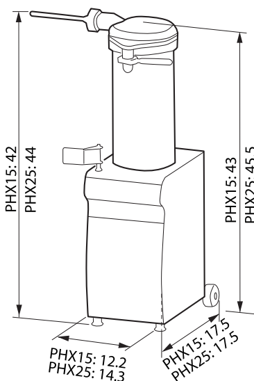
Dimensions PHX15 & PHX25
